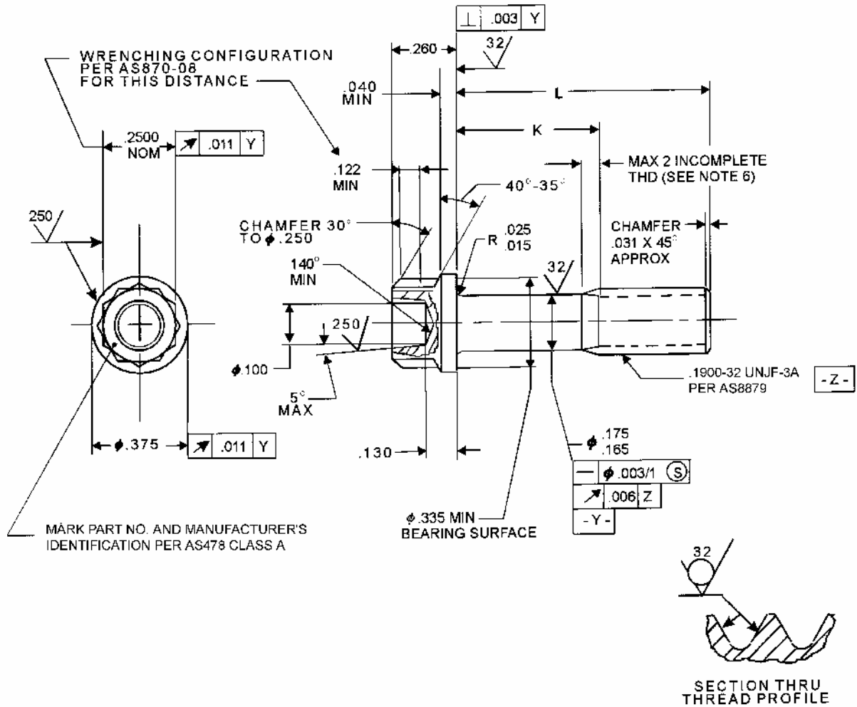
FIGURE 1 - BOLT
